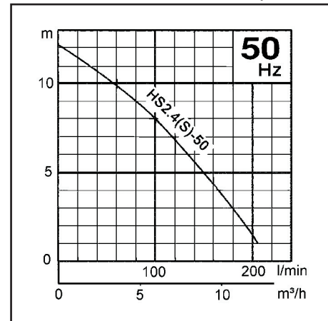
Pumpekurve
