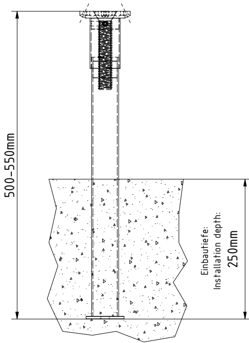
Installation depth of the Pedix B500 & Pedix B500+50
