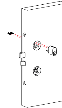
Step 2. Assemble the cylinder
