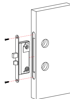
Stap 1. Monteer de pen
