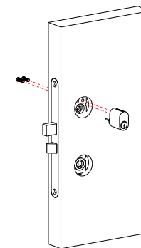
Stap 2. Monteer de cilinder
