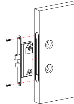
Step 1. Assemble the mortise
