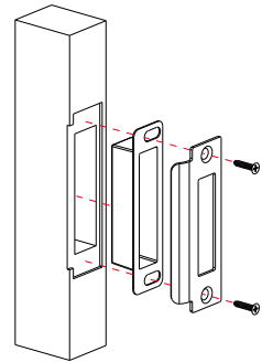
Step 3. Drill hole for strike plate/box
