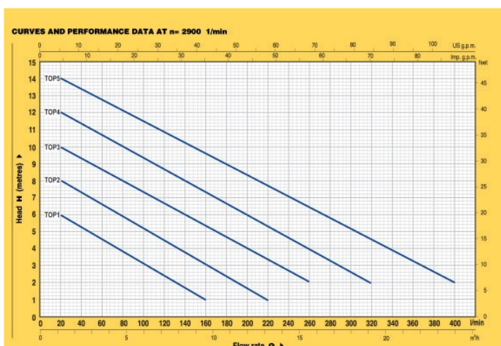
Pumpekurve
